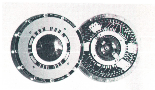
Fig. 14. The membrane probe for DAC testing.
