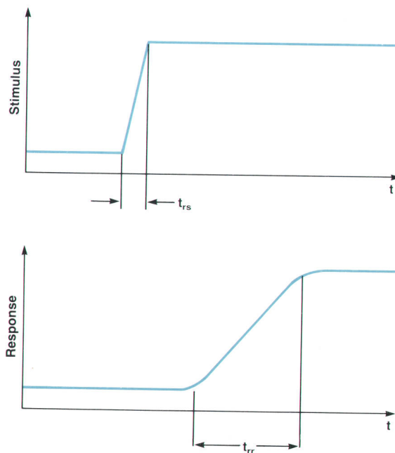
Fig. 3. The effect of parasitic inductance in the time domain.
